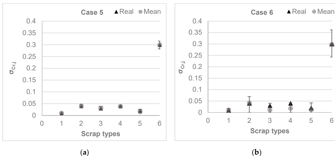
Figure 3. Estimated mean standard deviations for concentration of Cr ( \bar{\sigma}_{Cr} ) with a 95% confidence interval in six scrap types, x1–x6 for cases 5 and 6, (a,b).
