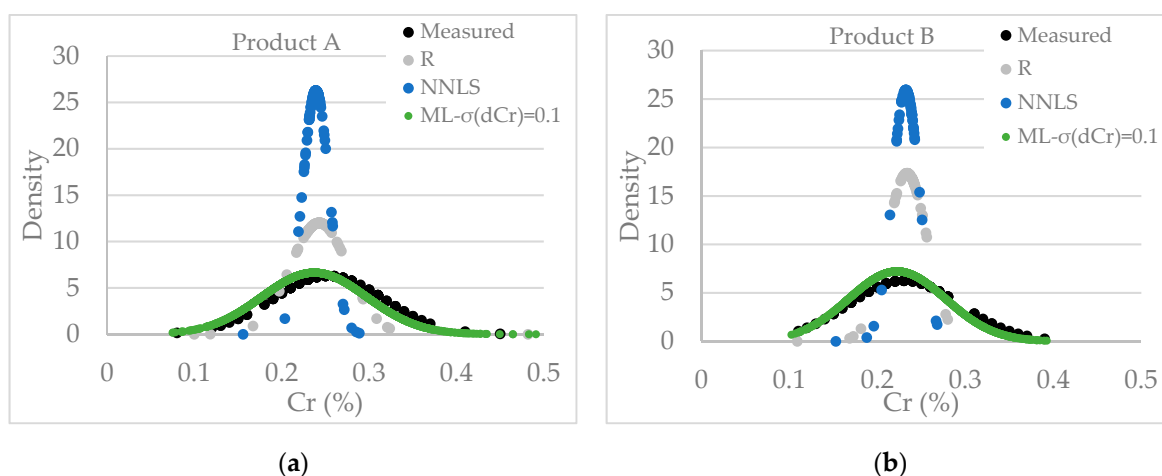
Figure 7. Comparison between the reported Cr concentration and calculated ones in scrap (x1–x10).
