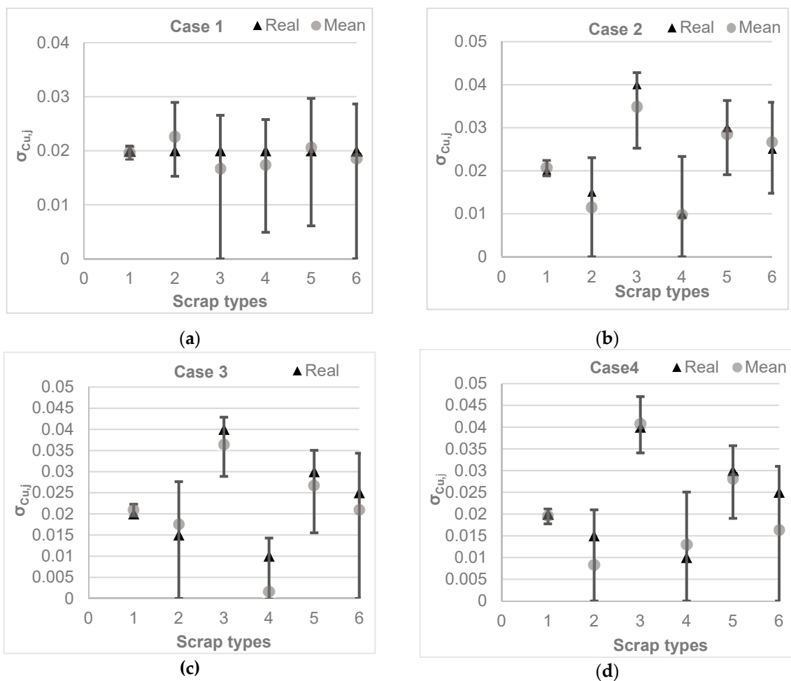
Figure 2. Estimated mean standard deviations for concentration of Cu ( \bar{\sigma}_{Cu} ) with a 95% confidence interval in scrap types, x1–x6 for cases 1–4, (a–d).
